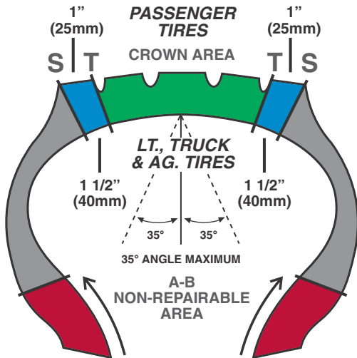
Uni-Seal Ultra repairs are designed for use in the Crown (T-T) area of the tire only.
